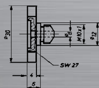
Plate nosepiece PA with cut-out: For standard blind rivets (Dome head)
